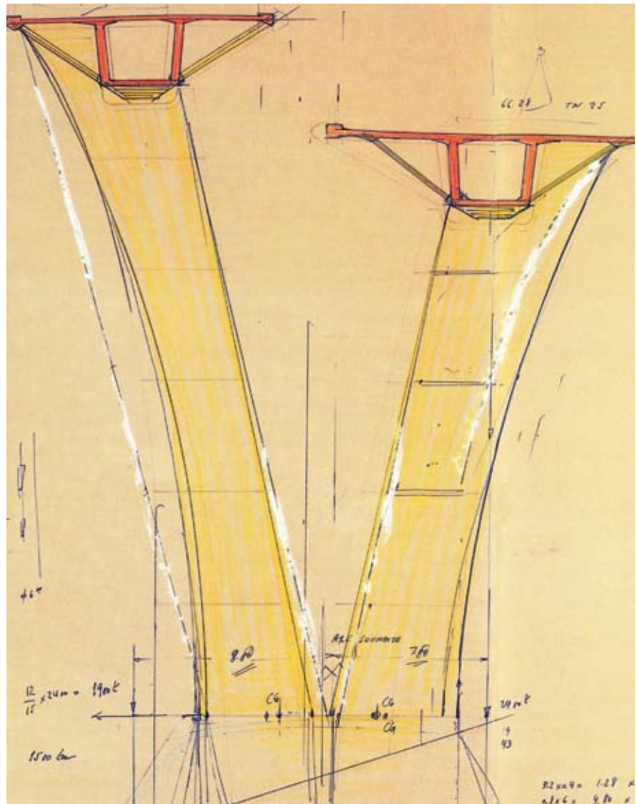
Fig. 23. This is a design sketch of the Rogerville Viaduct in France.
